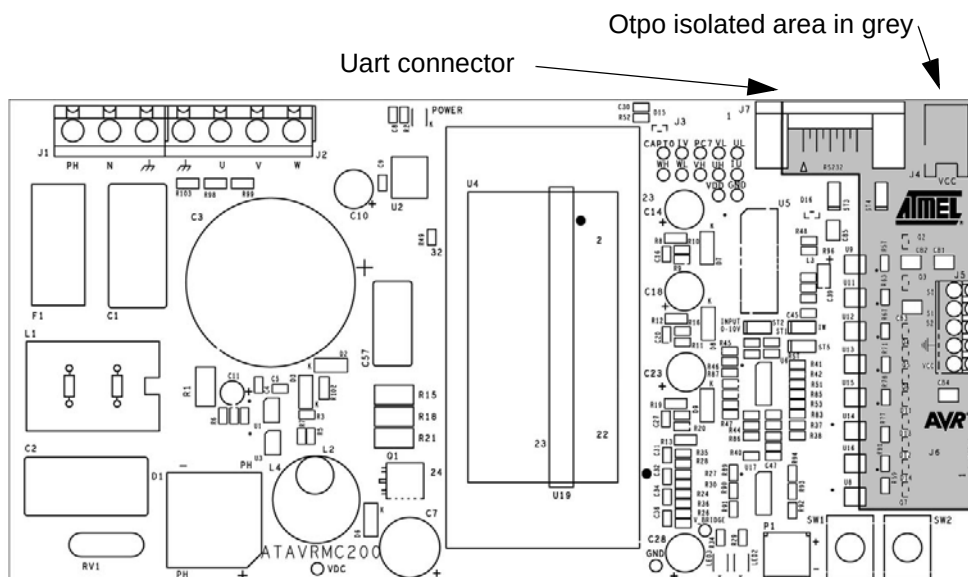
Figure 3-5 . Position of opto isolated area and uart connector
